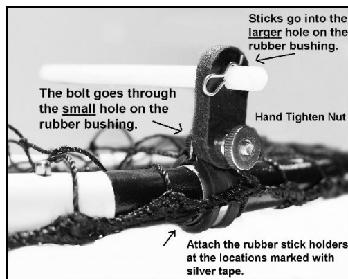
Stick Holder Attachment
