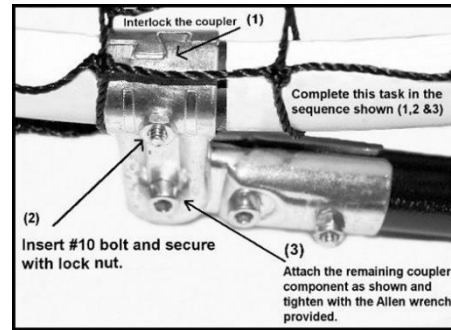
Sequence for ease of Assembly
