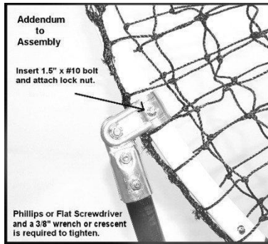
Additional Bolt for Stability
