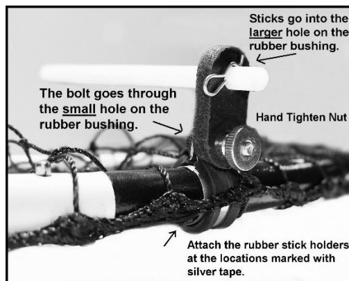
Stick Holder Attachment
